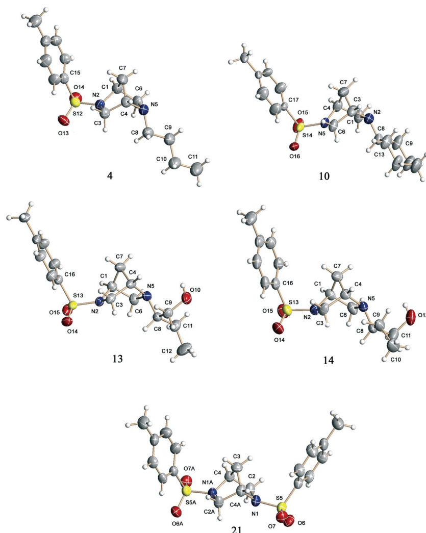
Figure 1. X-ray crystallographic structures and solid-state conformations of 4 , 10 , 13 , 14 , and 21 . [19]
